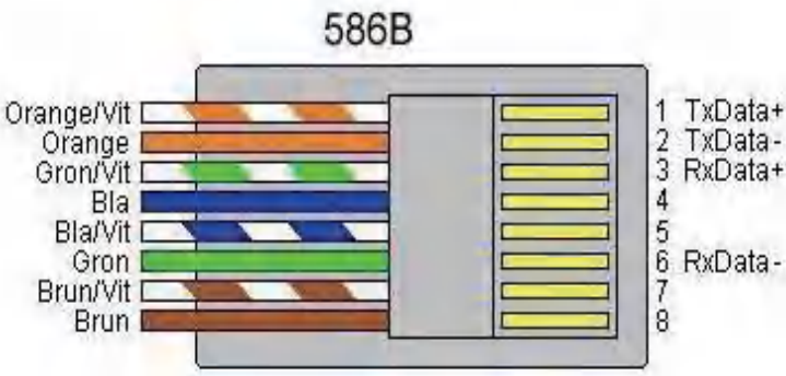
Figure 9. Network terminal Harness
